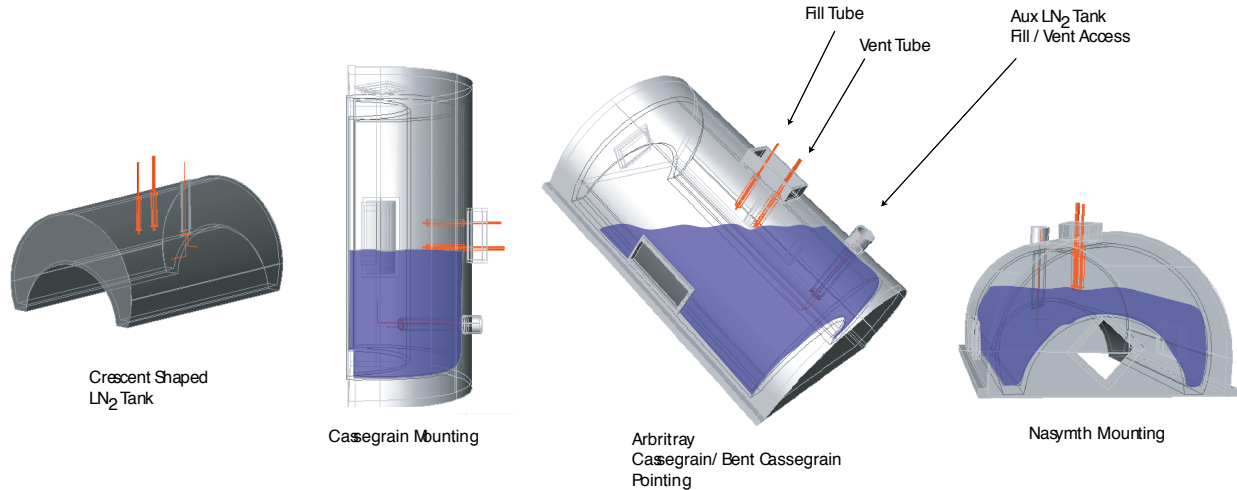
Figure 7. Schematic of the crescent shaped LN 2 tank. Tank size and tube placement allows use of the Dewar at either Cassegrain, Bent-Cassegrain, or Nasmyth telescope mounts without spillage. A nominal fill of 40% capacity will give at least a two-day hold time.
